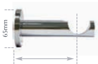
Strand 7cm Bracket
